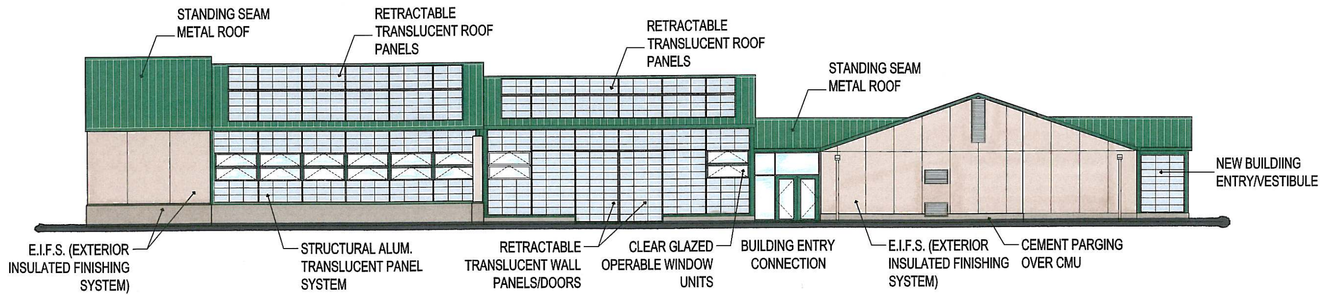
KING COUNTY POOL - SOUTH ELEVATION
